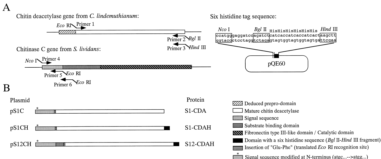
Fig. 1. Construction of recombinant chitin deacetylases. A: Origins of the fragments for the construction of fusion proteins and the positions for PCR amplification. The positions of oligonucleotide primers are indicated by arrows. B: Molecular architecture of the proteins used in this study.
