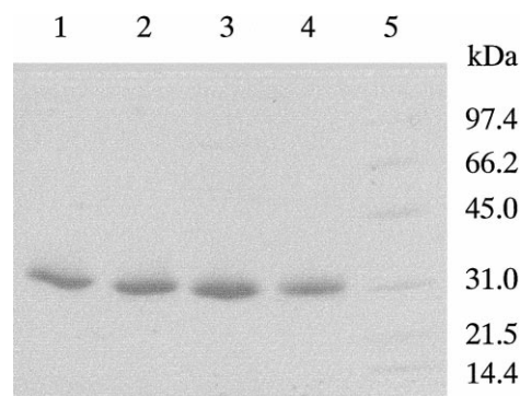
Fig. 3. SDS-PAGE of purified recombinant chitin deacetylases. Lane 1, S12-CDAH; lane 2, S1-CDAH; lane 3, S1-CDA; lane 4, the original chitin deacetylase from C. lindemuthianum ; lane 5, molecular mass standards (SDS-PAGE Molecular Markers Low-range, Bio-Rad, USA.)
